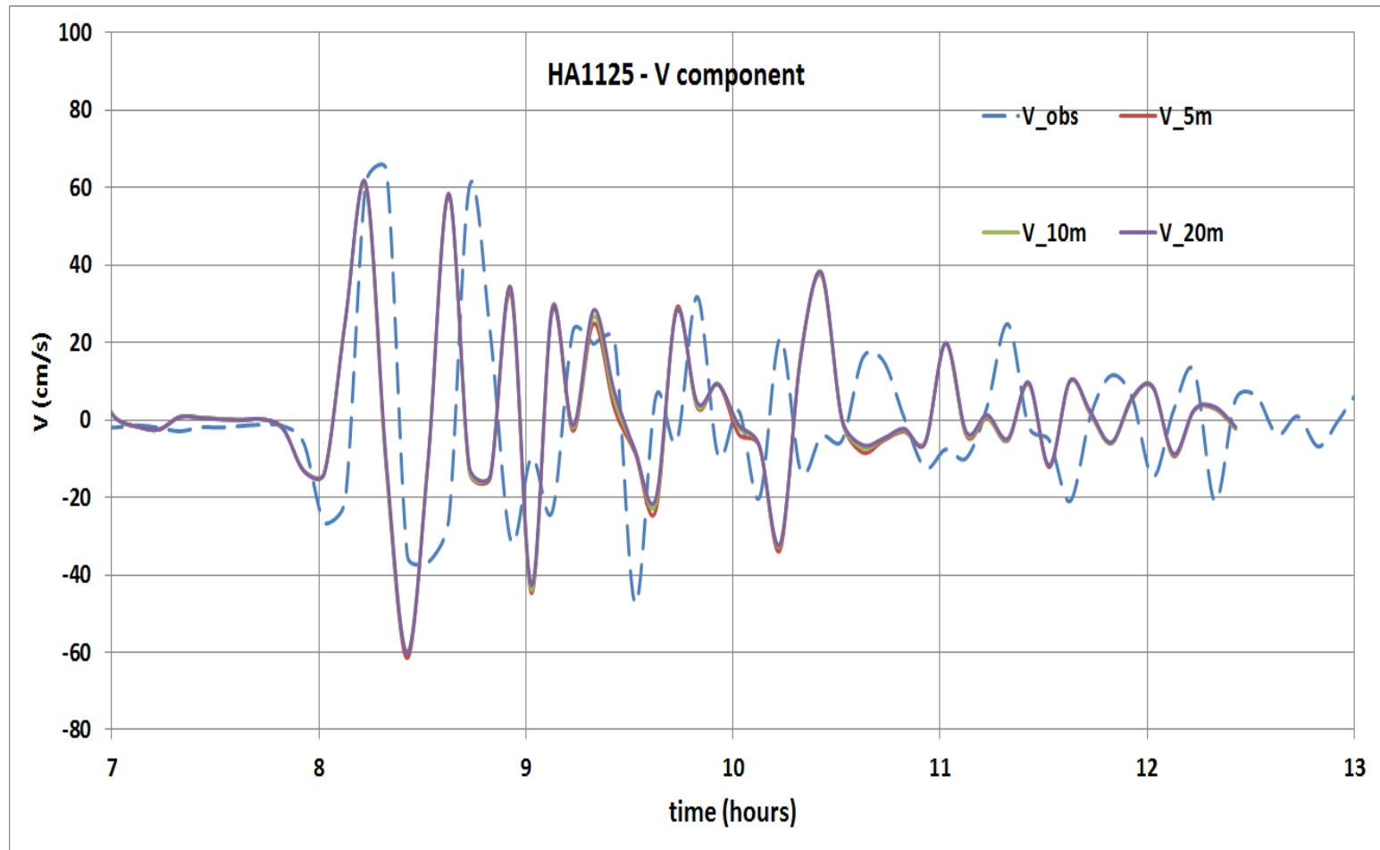
HA1125 – V component (detided dashed line)
